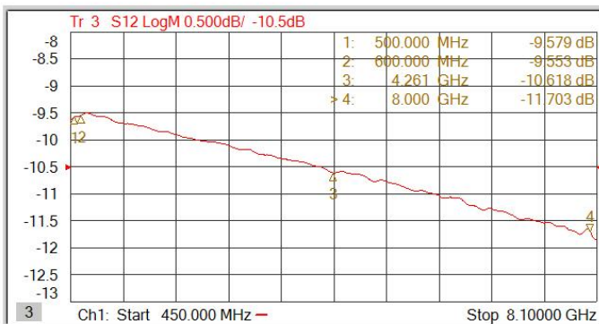
图3:插入损耗
